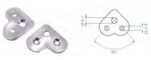
Top 90° graders
