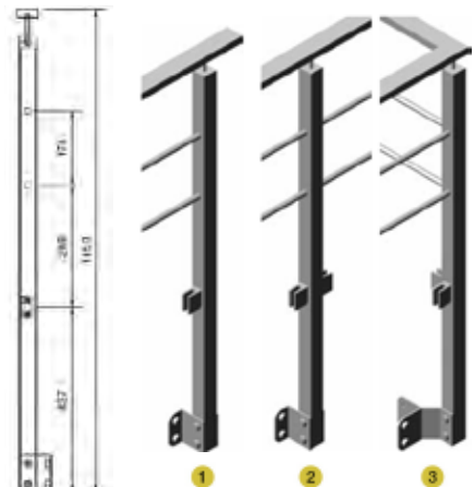
Side monteret 40.302
