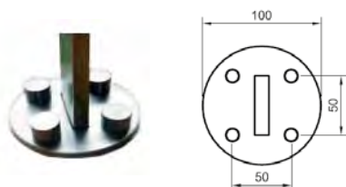
Standart fod for B-inox 320
