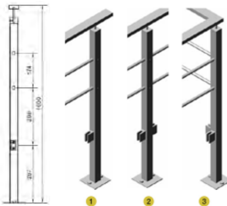
Top monteret 40.302
